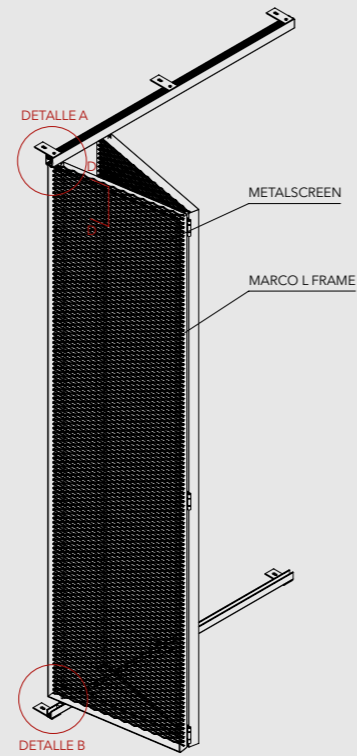
FOLDING L FRAME - METALSCREEN
