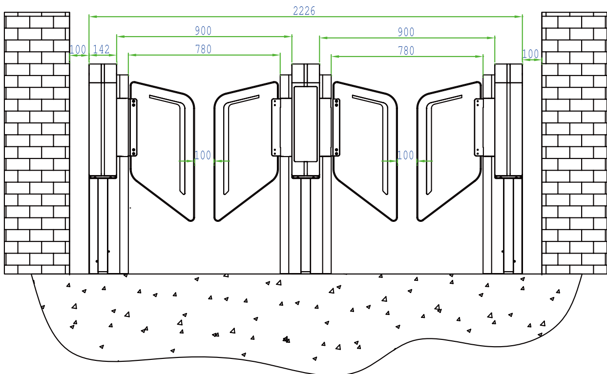
Figure 2-1 SBTL9000 Series Dual-lane
